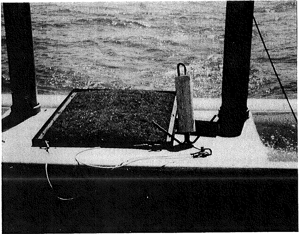
FIGURE 1. The artificial substrate, frame, and anchor used to collect white sturgeon eggs in the Columbia River downstream from Bonneville Dam.
