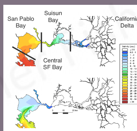
Maps of the northern San Francisco Estuary showing regions and boundaries (black lines). Modeled depth- and daily-averaged salinity for two steady flow scenarios. Top: 340 m 3 s -1 . Bottom: 1,440 m 3 s -1 , close to the 20th and 80th percentiles, respectively, of monthly mean Delta outflow from water years 1956 through 2011. (Kimmerer et al. 2013)
